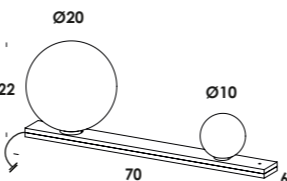
nash 70/lp2 dim on/off touch E27 max 60w - 230V G9 max 40w - 230V compatibile con lampade classe C→A+ compatible with lamps class C→A+
