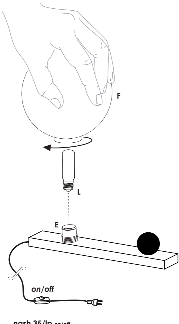
nash 35/lp on/off
