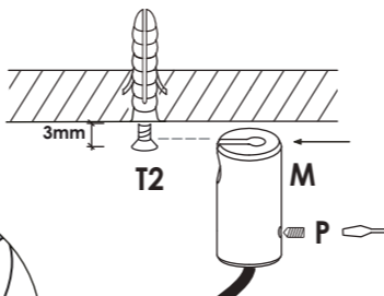
fig.2 - acc. terminale cavo acc. terminal for cable
