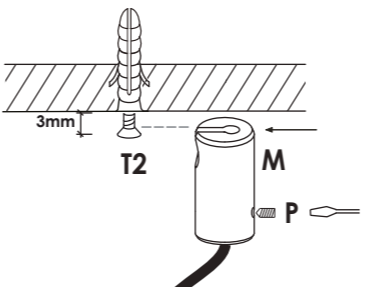
fig.2 - acc. terminale cavo acc. terminal for cable
