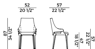
942/7 sedia \ chair
