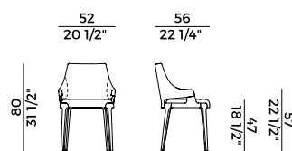
942 sedia \ chair
