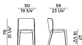
902 sedia \ chair
