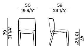
902 sedia \ chair
