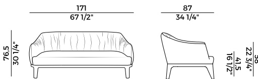
840/D divano \ sofa
