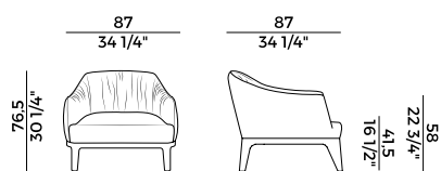
840/PL lounge \ lounge armchair
