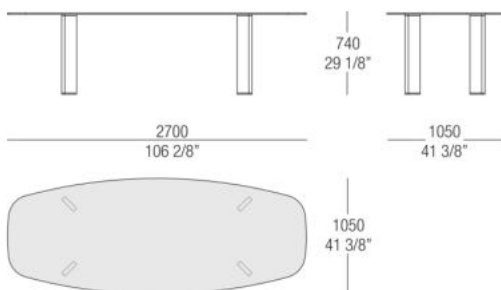
Oval table with glass top
