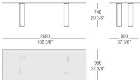
Rectangular table with glass top
