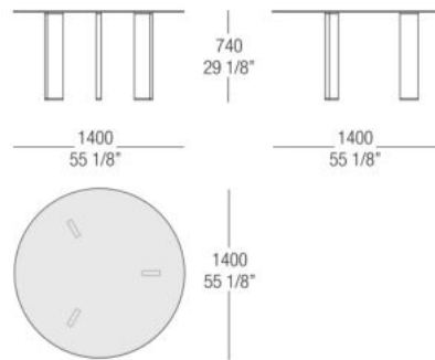
Round table with glass top
