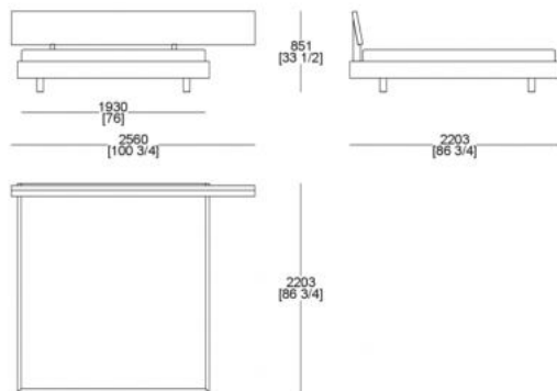
Customer bedspring (mattress W. 1930 x D. 2020 mm)
