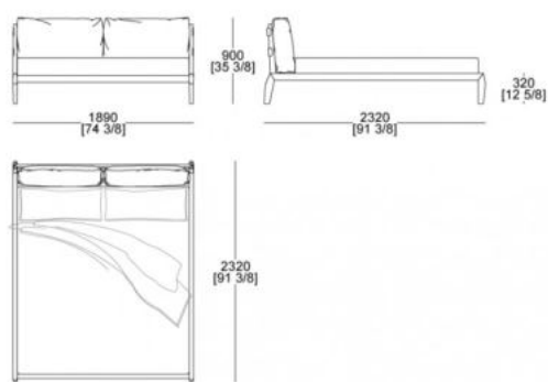
Bed (mattress W. 1800 x D. 2000 mm)
