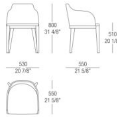
Low backrest chair with armrests
