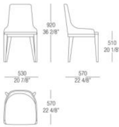
High backrest chair
