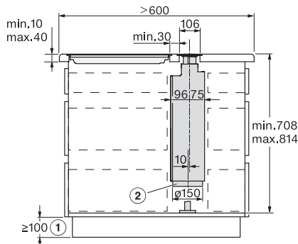
DAD4840, DAD4940 - flush - side view - Installation drawings
