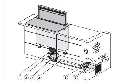
DAD4840, DAD4940 - DUP150, Installation version 1, Installation drawings
