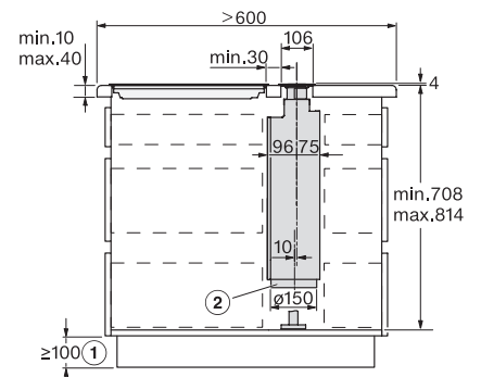
DAD4840, DAD4940 - surface mounted, AP > 600 mm - side view - Installation drawings
