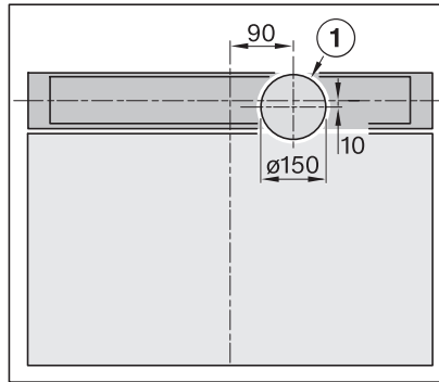
DAD4840, DAD4940, flush AP > 600 mm, Top view, Installation drawings
