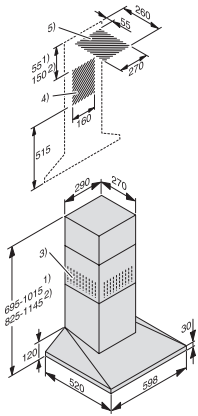
DA 396-6 (Installation drawing)
