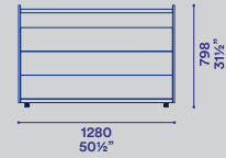
contenitori P 511 / drawer unit D 21 1/4"
