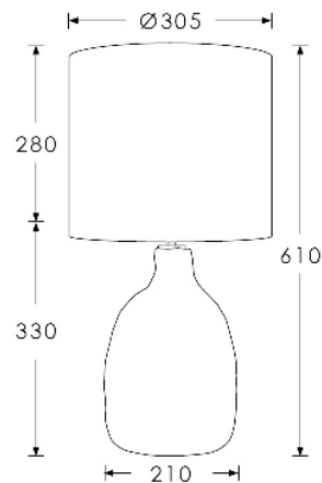
Dimensions in mm and approximate
