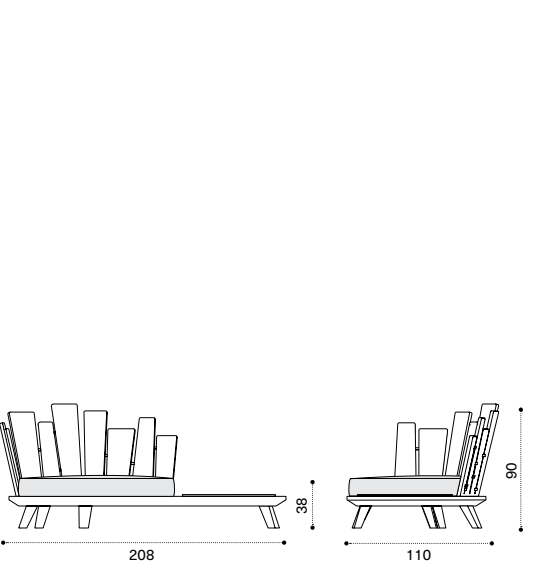
Lounge armchair right with integrated coffee table
