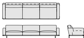
RB_3 - RB_3C cm. 300x87,5x43,5/72,5h inch 118 1 / 4 x34 3 / 4 "x17 1 / 4 /28 1 / 2 h
