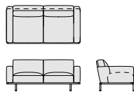
RB_2S - RB_2SC cm. 170x87,5x43,5/72,5h inch 67 1 / 4 x34 3 / 4 "x17 1 / 4 /28 1 / 2 h
