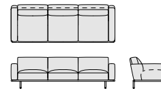
RB_3S - RB_3SC cm. 240x87,5x43,5/72,5h inch 94 1 / 2 x34 3 / 4 "x17 1 / 4 /28 1 / 2 h
