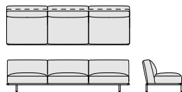
RB_5 - RB_5C cm. 270x87,5x43,5/72,5h inch 106 1 / 4 x34 3 / 4 "x17 1 / 4 /28 1 / 2 h
