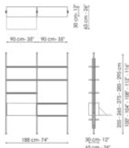
Ceiling fixing 2 modules Width: 188cm Depth: 30cm Height: 255-265-275-285-295cm
