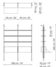
Wall fixing 2 modules Width: 188cm Depth: 33cm Height: 240cm
