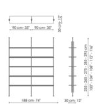
Ceiling fixing 2 modules Width: 188cm Depth: 30cm Height: 255-265-275-285-295cm
