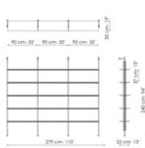
Wall fixing 3 modules Width: 280cm Depth: 33cm Height: 240cm
