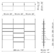
Ceiling fixing 3 modules Width: 280cm Depth: 30cm Height: 255-265-275-285-295cm
