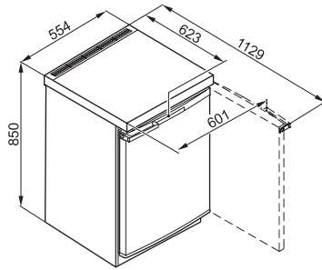
F12011S, F12011S-1 F12011S-2 (installation drawings)
