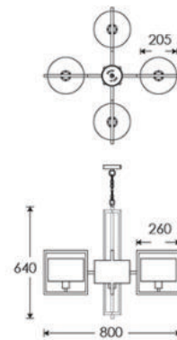
Dimensions in mm and approximate *Adjustable flex and chain length
